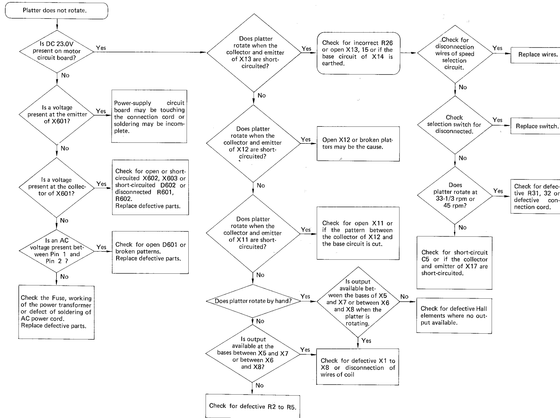
9-(1) Chart 1. "Platter does not rotate"
